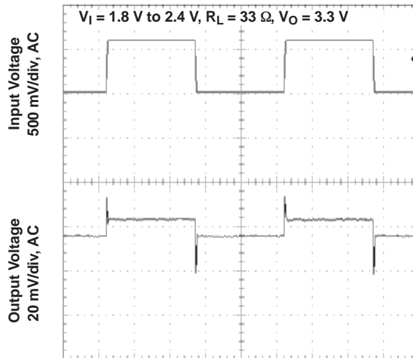
t – Time – 2 ms/div Figure 16.
