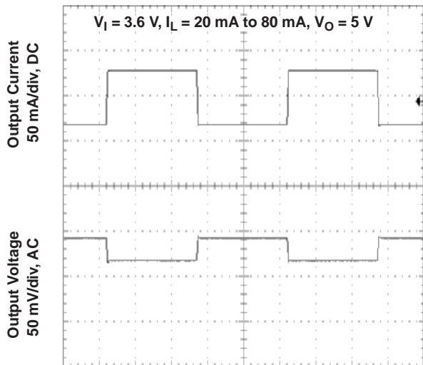
t – Time – 2 ms/div Figure 15.
