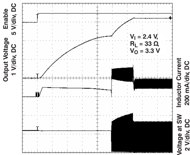
t – Time – 200 μs/div Figure 18.
