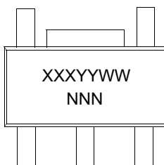
3-Lead SOT-223
